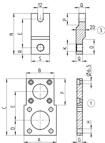
Hydrocheck connecting kit to suit cylinders Ø 40 - 50 - 63 - 80 mm
